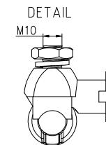
HV BUSHING TERMINAL
