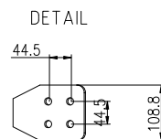
LV BUSHING TERMINAL
